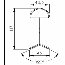
HD Roll Formed Post Overhead View
